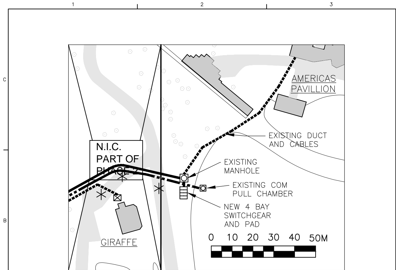
① PART DWG. SP-01 - DETAIL 6 Scale: NO SCALE
